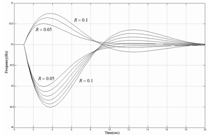
Fig. 7 Frequency Response for Varying Values of R (0.05-0.1)
