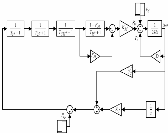
Fig. 1 Typical Reheat Turbine Governor Model
