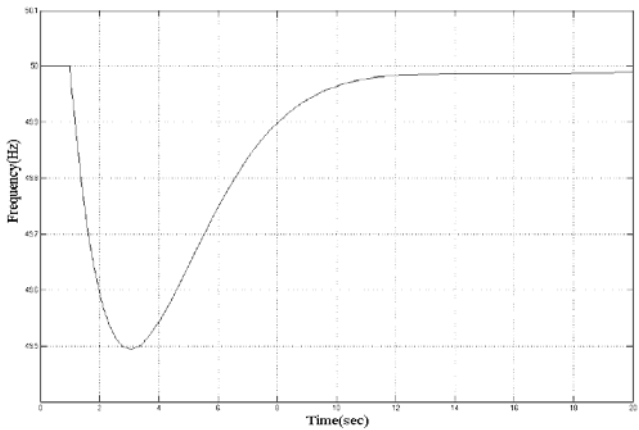
Fig. 5 System Frequency Response to Step Disturbance Input
