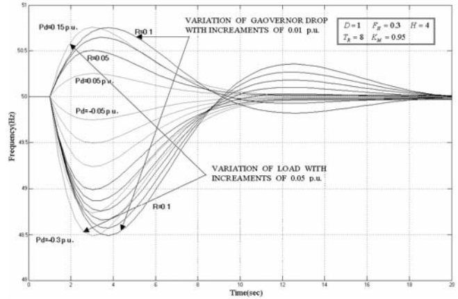
Fig. 12 System Frequency Response with Consideration on Load and Governor Droop
