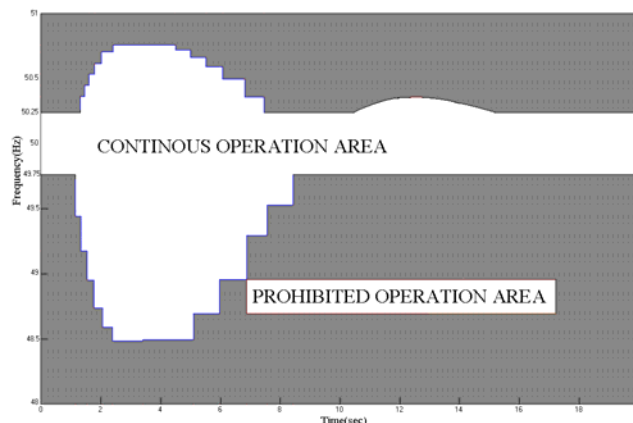
Fig. 14 Six Steps Setting Corresponding Frequency Relay
