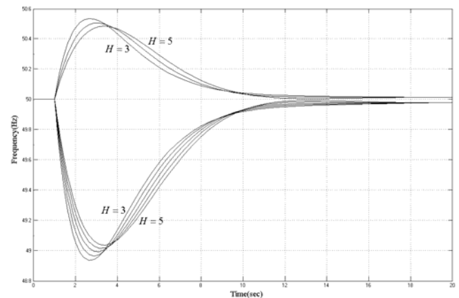
Fig. 8 Frequency Response for Varying Values of H (3-5)
