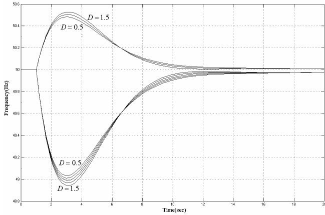
Fig. 9 Frequency Response for Varying Values of D (0.5-1.5)
