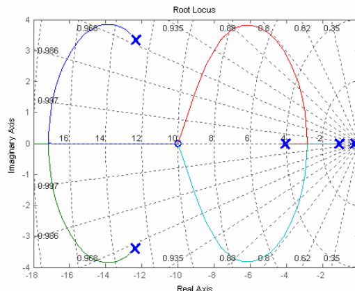
Fig. 2 Corresponding root locus of power plant model
