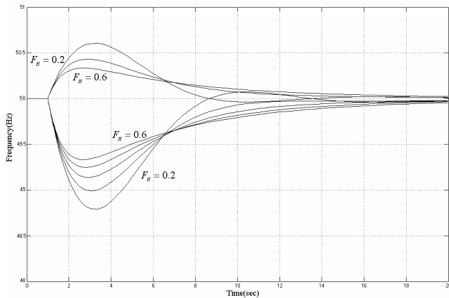
Fig. 11 Frequency Response for Varying Values of FH (0.2-0.6)
