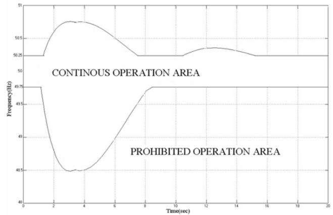
Fig. 13 Sheath of System Frequency Response with Consideration on Load and Governor Droop
