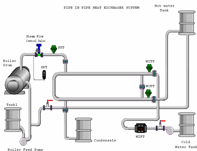
Fig. 1 Mimic diagram of heat exchanger pilot plant
