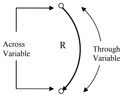
Fig. 2 Linear graph representation of a resistor
