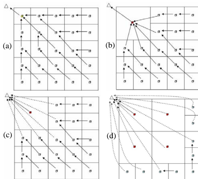
Fig. 7 The operation of cluster merging mechanism
