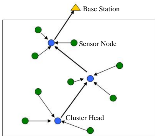
Fig. 1 A clustered wireless sensor network
