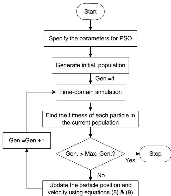
Fig. 5 Flowchart of particle swarm optimization algorithm
