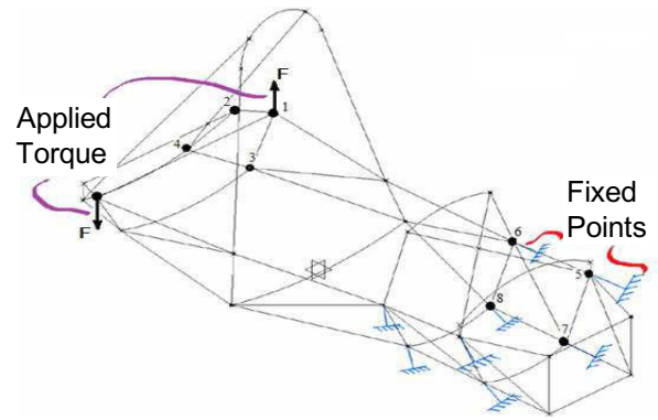
Fig. 4 Model for FEM analysis
