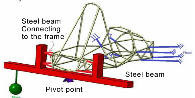
Fig. 5 Model for experiment setup
