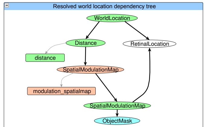
Fig. 7. By incorporating knowledge already acquired by the system, the structure of the effective dependency graph changes and its size shrinks.
