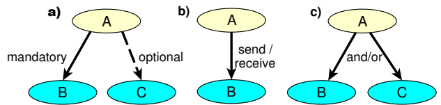
Fig. 3. We cover different cases using modifiers for a dependency link pattern: a) dependencies can be optional or mandatory, b) different operations (send and receive) are requested for the target node and c) we differentiate between the need for all dependencies or only one-of-many dependencies to be fulfilled.
