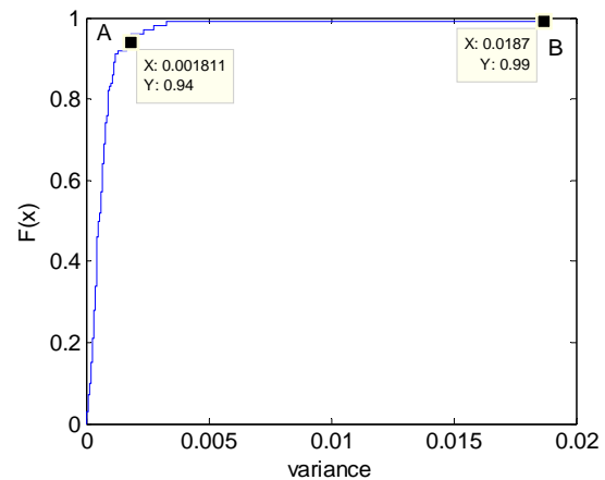
Fig. 5 CDF of variance between AS and DM
