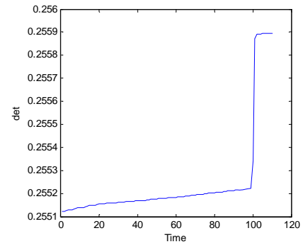
Fig. 7 Metric \delta_{RTT} changes with network congestion
