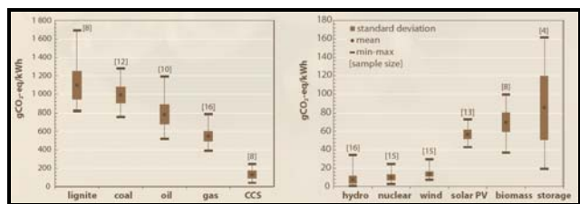
Fig. 1 Greenhouse Gas Emissions (g Ceq per kWh)
