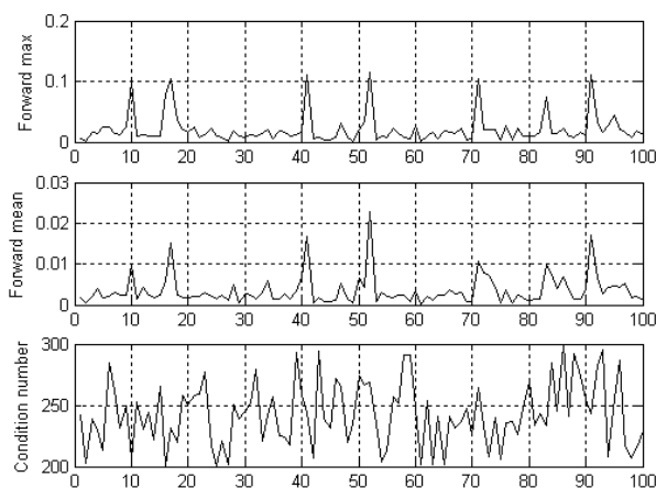
Fig. 6 Forward Error and Condition Numbers
