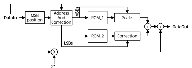
Fig. 4 LUT Architecture
