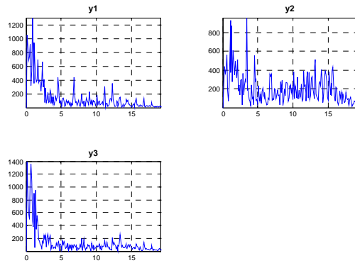
Fig. 6. FFT diagram for Normal Rhythm
