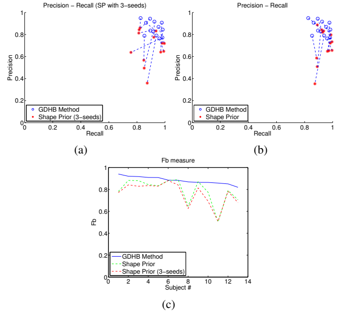
Fig. 6. Comparisons based on Precision vs Recall diagrams and the F_1 /Dice coefficient. In (a) and (b) results of the two methods are connected with dashed lines to show the improvement the proposed method achieved.
