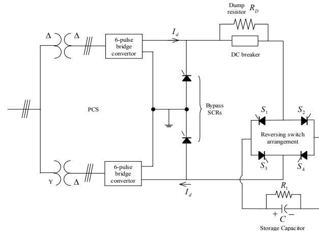
Fig. 2 Capacitive Energy Storage Unit
