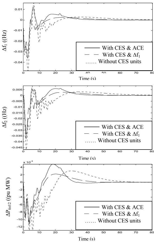
Fig. 4 Dynamic responses for \Delta f_1 , \Delta f_2 and \Delta P_{tie12} considering a step load disturbance of 0.01 pu in area-1.
