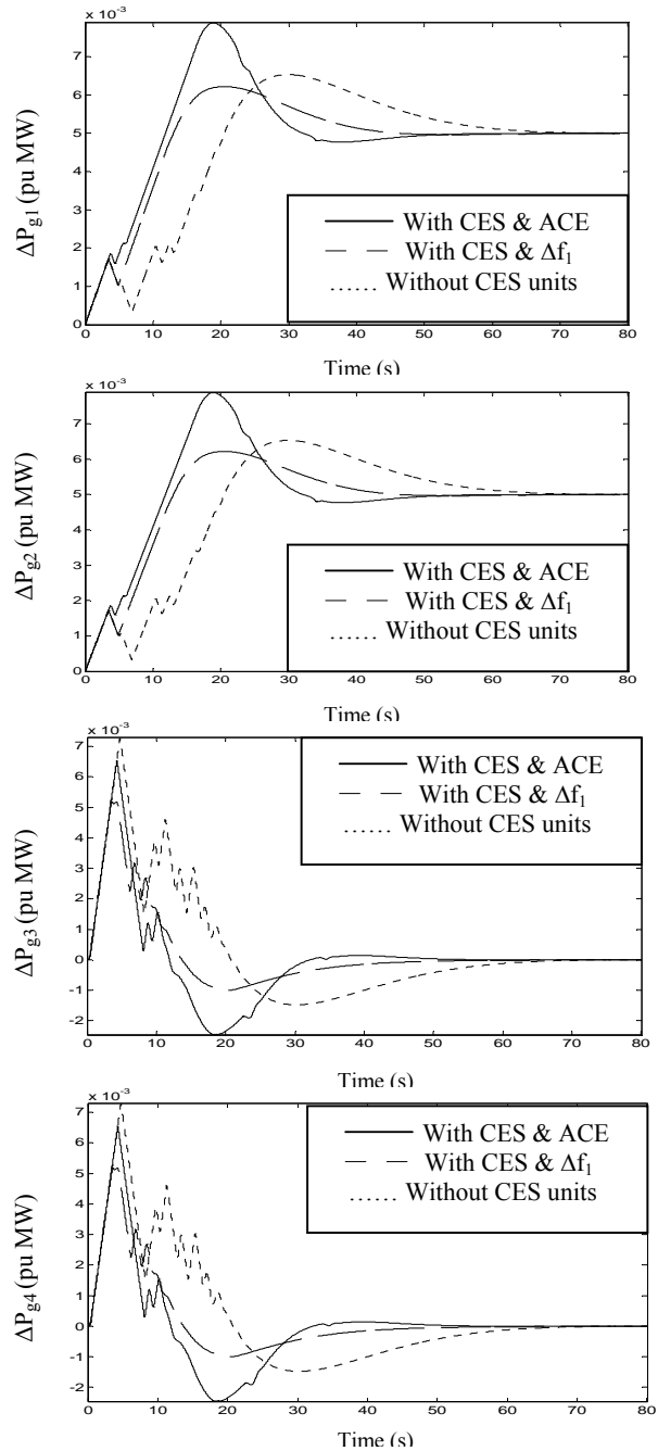
Fig. 5 Dynamic responses for \Delta P_{g1} , \Delta P_{g2} , \Delta P_{g3} and \Delta P_{g4} considering a step load disturbance of 0.01 pu in area-1.
