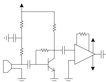
Fig. 9 Circuit of a stereo microphone system
