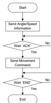
Fig. 11 Flowchart of commands for motor control
