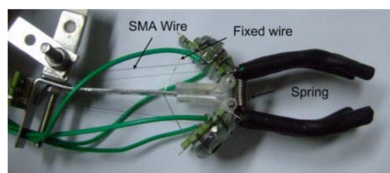
Fig. 7 Gripper structure of a pipe robot
