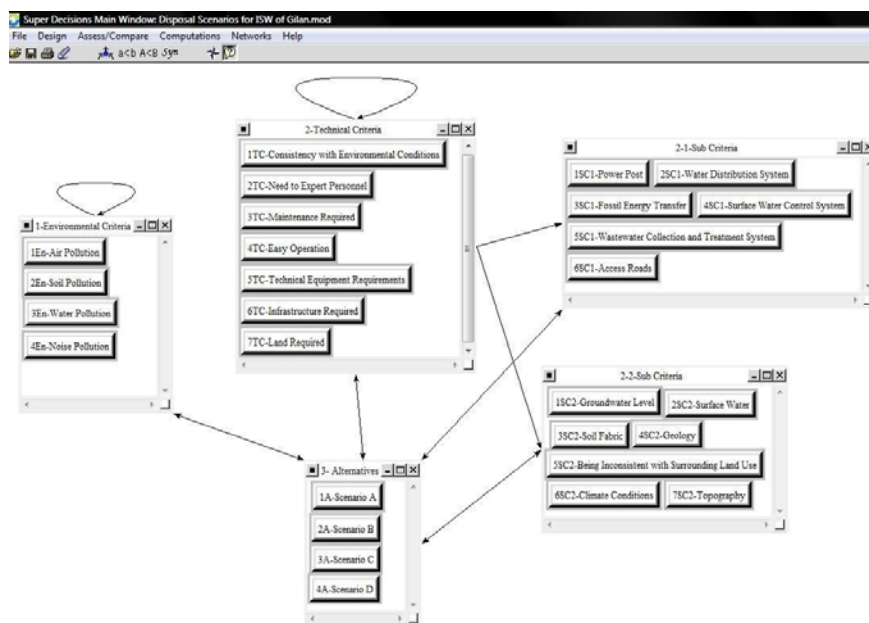
Fig.8 Super Decisions model
