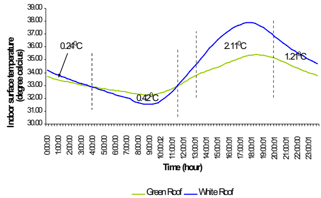
Fig. 9 (d): Comparison of average indoor surface temperature between green roof and white roof for six days' reading.
