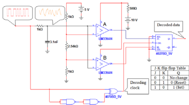
Fig. 5 Indicates the final stage of the Decoder; the output of Comparators A and B are connected with J-K ff in Ports J and K respectively; the Clear and Set ports are connected to the ground
