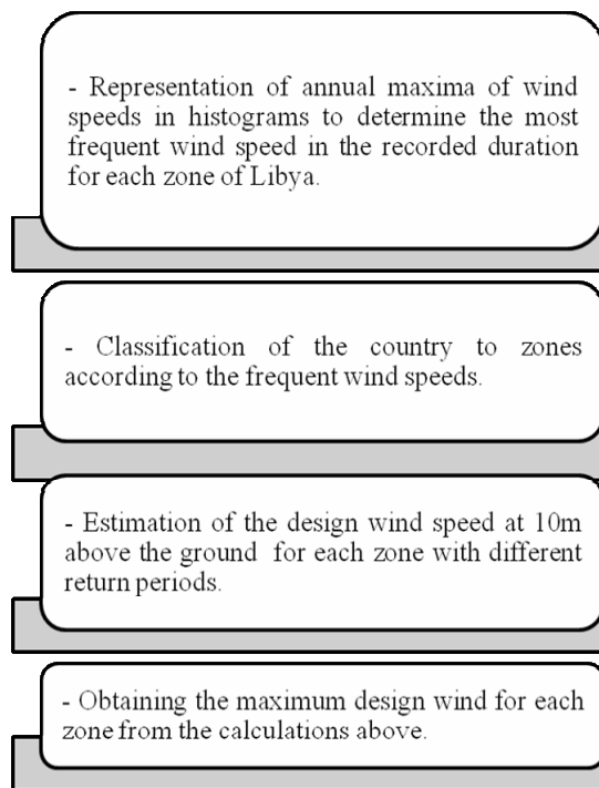
Fig. 1 Flowchart of wind speed data analysis
