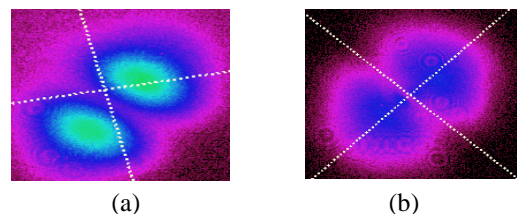
Fig. 4 (a) Near field and (b) Far field of TEM01 mode, r=0.89\text{ mm} , z=7.7\text{ mm}
