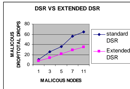
Fig. 4 Percentage of malicious drops over total drops
