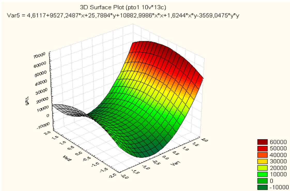
Fig. 2 Response surface of the second order model.
