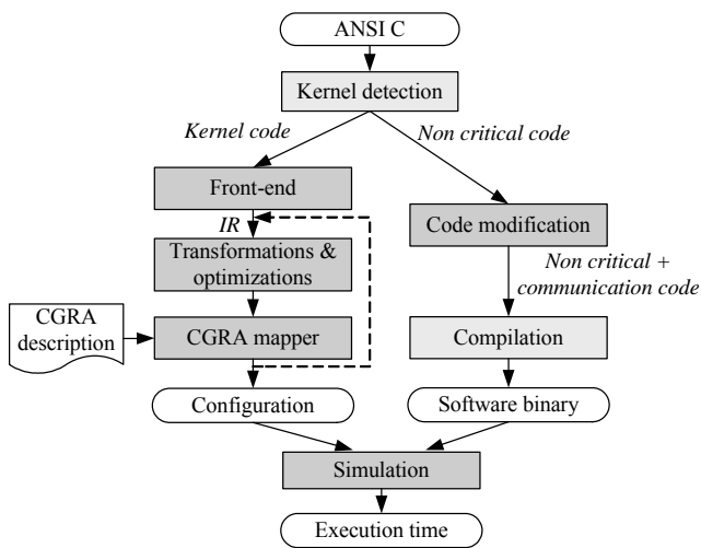
Fig. 4 Design flow for microprocessor/CGRA systems
