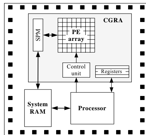
Fig. 1 Overview of the reconfigurable SoC platform
