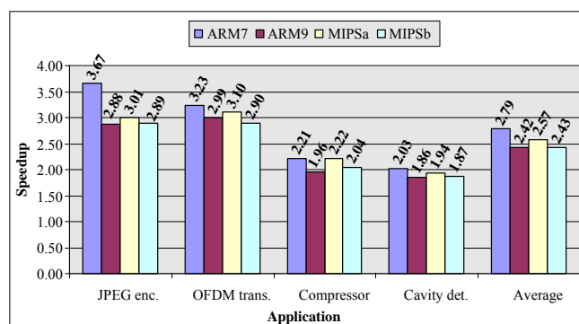
Fig. 6 Application speedups for the processor/CGRA2 SoCs
