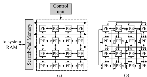
Fig. 2 (a) Outline of a CGRA architecture, (b) Point-to-point connectivity
