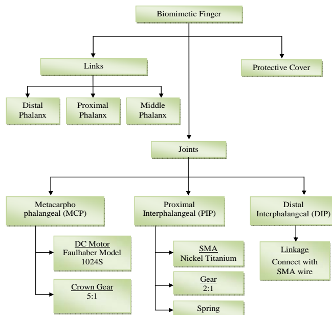
Fig. 4 Design concept of a hybrid actuation solution
