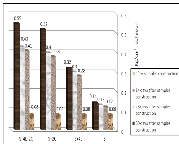
Fig. 2 Comparison of changes in cohesion on the different percentage of Lime and cement, at different times of processing
