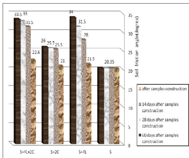
Fig. 1 Comparison of changes in Soil friction angle on the different percentage of Lime and cement, at different times of processing
