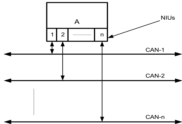
Fig. 10. Redundancy at network (CAN)
