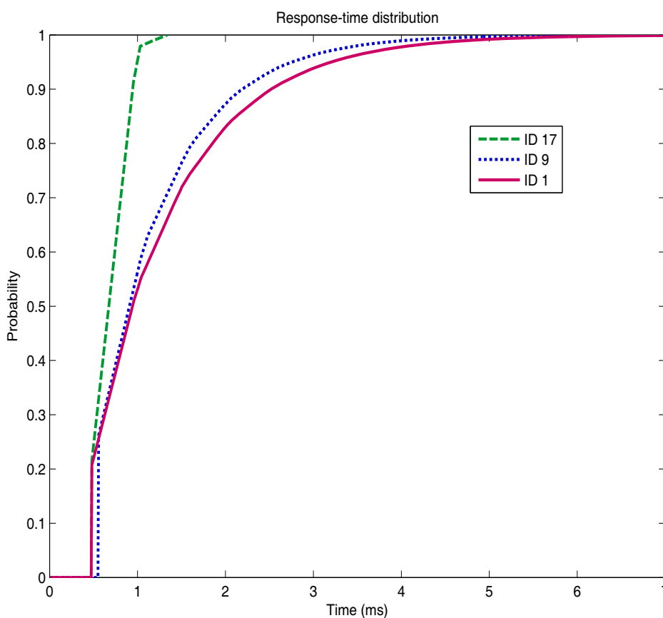
Fig. 8. Response-time distribution
