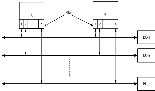
Fig. 11. Redundancy at network (MIL)
