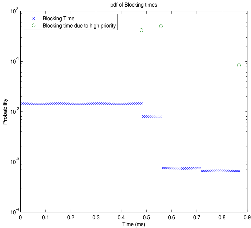
Fig. 7. pdf of blocking times
