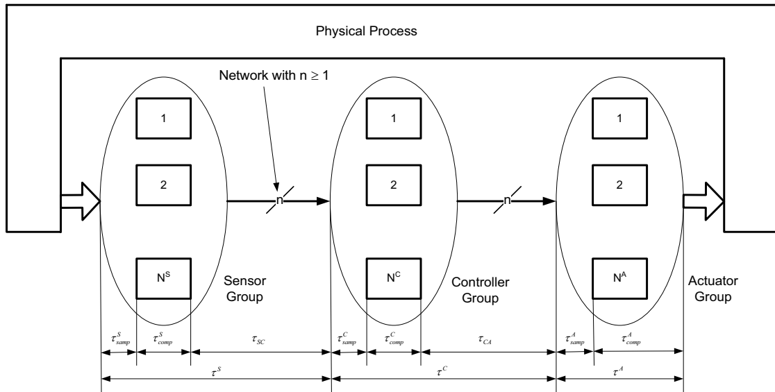
Fig. 13. NCS response-time with redundancies
