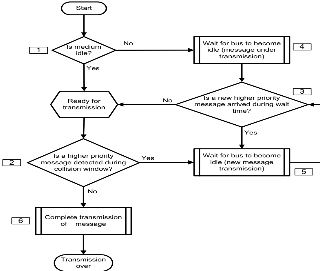
Fig. 6. Transmission procedure of CAN
