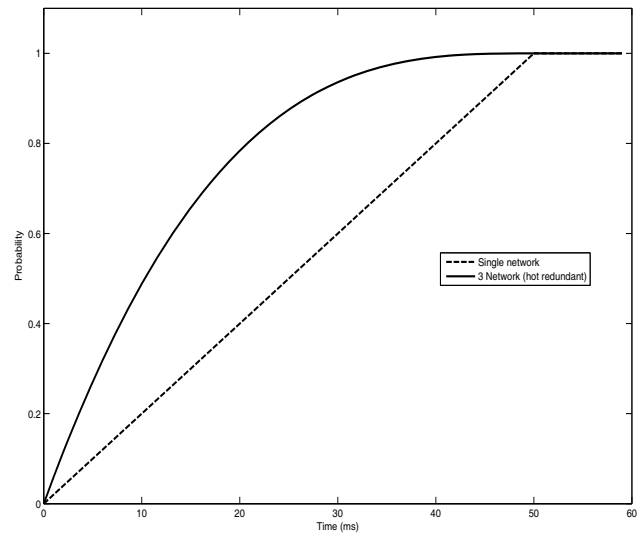
Fig. 12. Delay time distribution of data transfer
