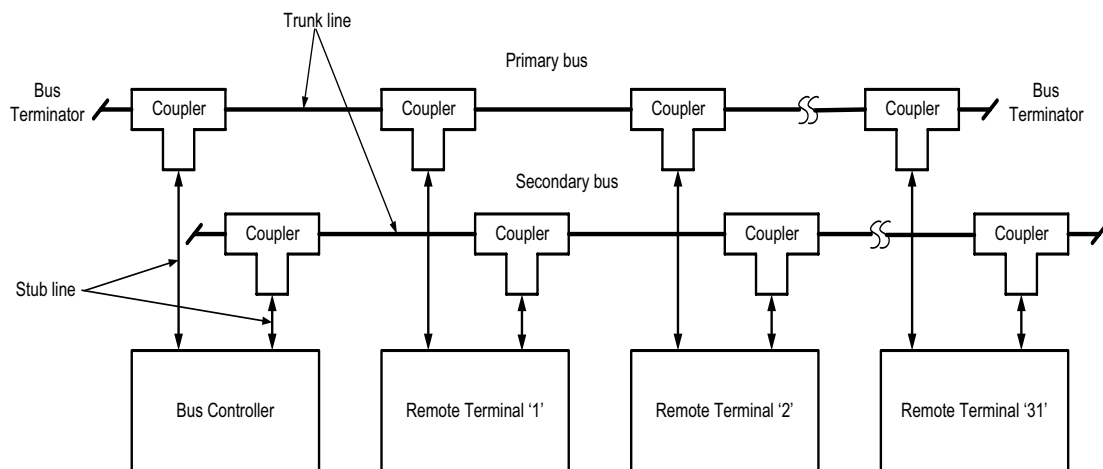
Fig. 3. MIL-STD-1553B network
