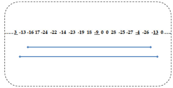
Fig. 2 Vertices and edges for marker -13 in A(Sc)
