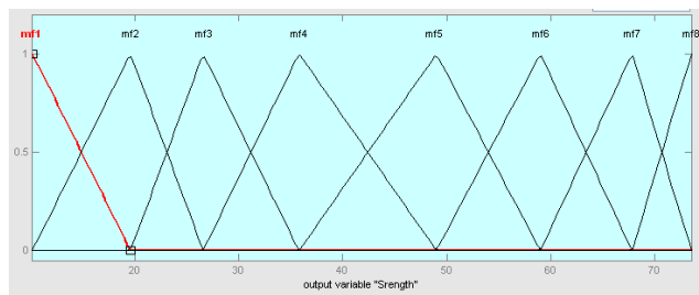
Fig. 5 Membership functions of output parameters (strength)
