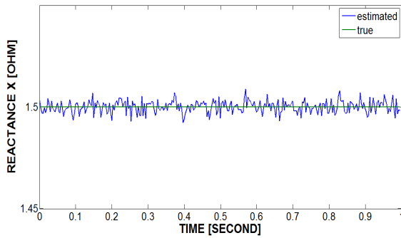
Fig. 6 Comparison between estimated and true value of parameter X
