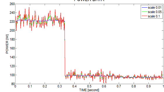
Fig. 4 Power data
