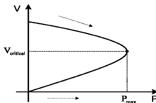
Fig. 1 PV curve
