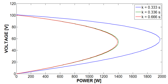
Fig. 10 Estimated PV curve at specified time k
