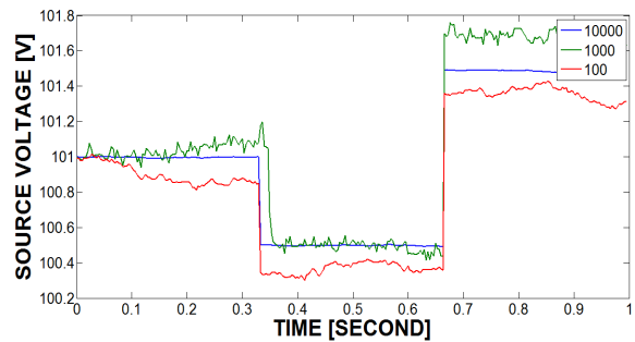
Fig. 11 Estimation with different number of particle
