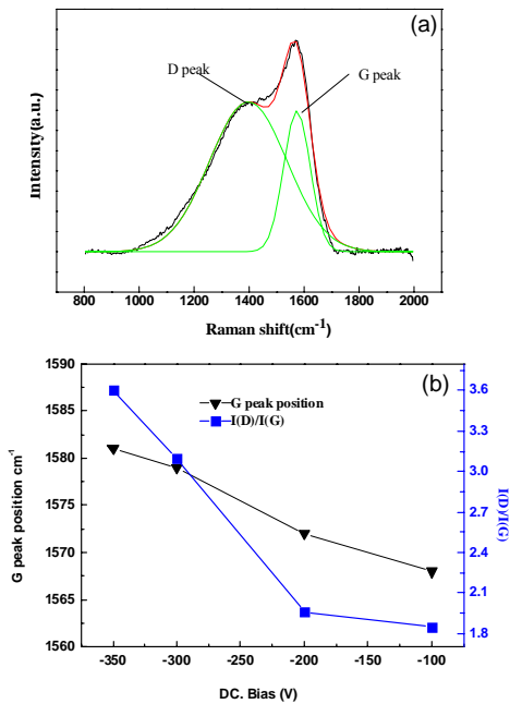
Fig. 1 Raman spectra of W- and S-doped DLC film. (a) Raman spectra of W- and S-doped DLC film at -300V. (b) G peak position and I(D)/I(G) ratio versus bias
