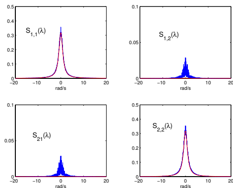
Fig. 4. Comparison between target and estimated spectrum
