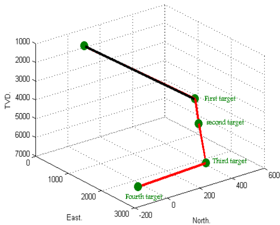
Fig. 9 Simulate Four Target Directional at First Target.
