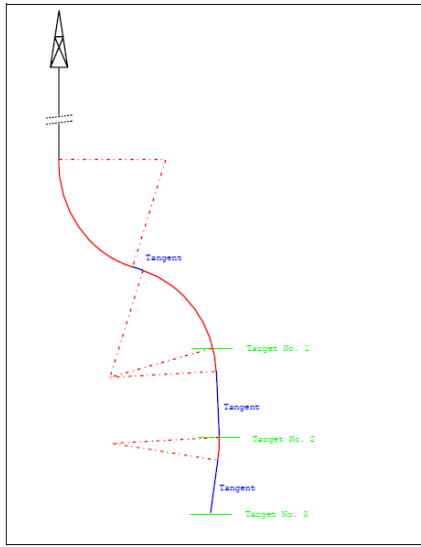
Fig. 7 Two Circular Arc Trajectory
