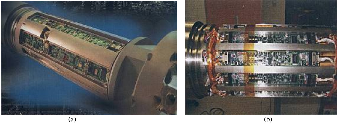
Fig.11 Non-Rotating Adjustable Stabilizer
