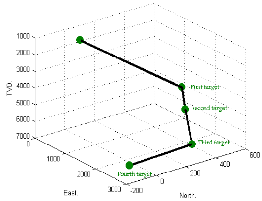
Fig. 10 Simulate Four Target Directional at Total Depth
