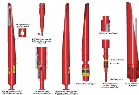
Fig. 2 Whip Stocks & Whip Stock Mills
