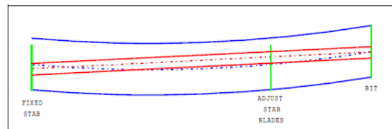
Fig. 5 Three-Point Geometry Contact Points
