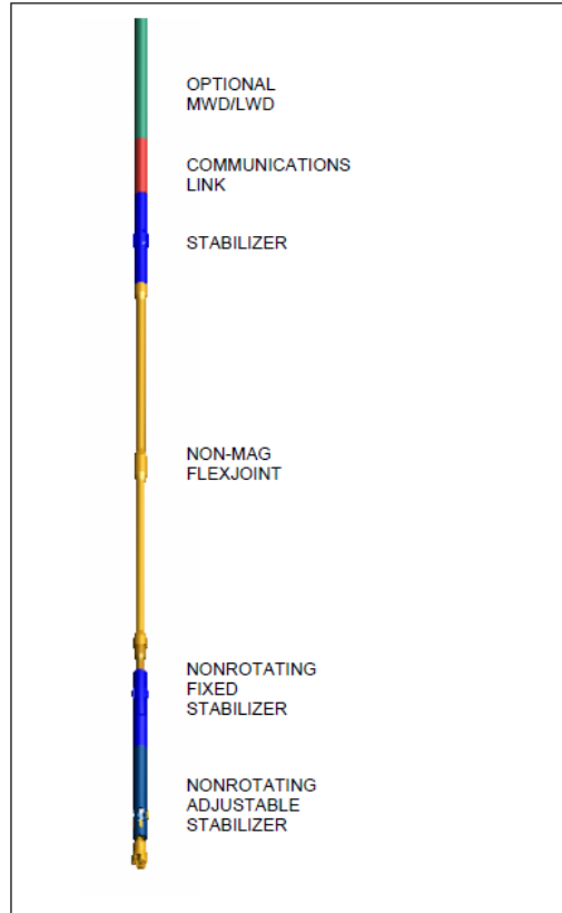
Fig. 4 NAS Bottom Hole Assembly
