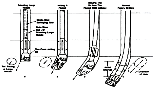
Fig. 1 Jetting bit technique
