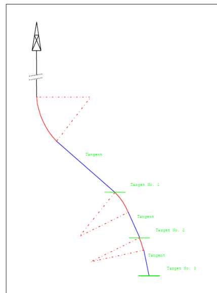
Fig. 6 Single Circular Arc Trajectories
