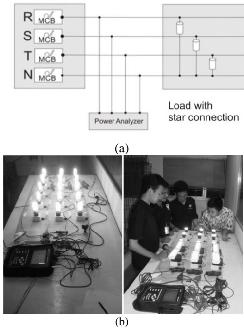
Fig. 2 (a) Star composition, (b) Test-bench
