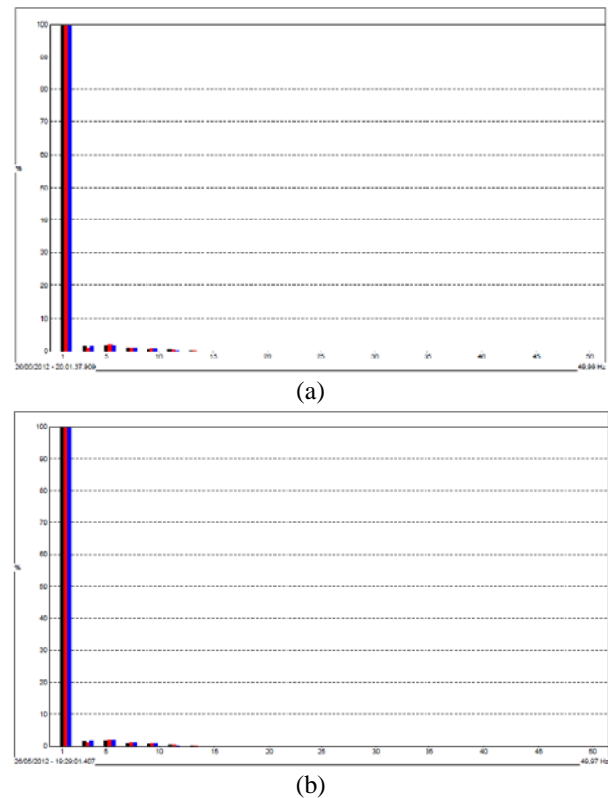
Fig. 4 Spectrum of voltage harmonic: (a) fluorescent, (b) WOLED
