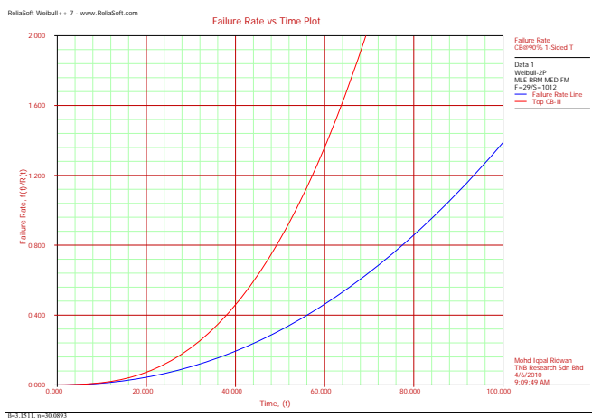
Fig. 4 Failure rate vs. Time From figure 4, it is observed that the failure rate of the relays increases over time. This indicates that the numerical overcurrent relays displayed a certain 'wear-out' characteristics during their life in service over a time period in TNB. This result is idem quod the engineering judgment made earlier which stated that the numerical overcurrent relays from Manufacturer A failed because of aging.
