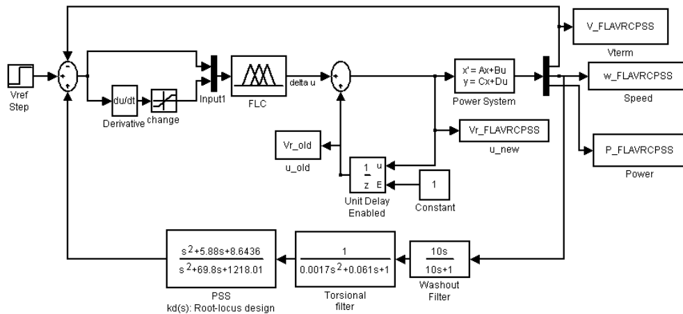
Fig. 10 SIMULINK diagram the system with FLAVR and CPSS
