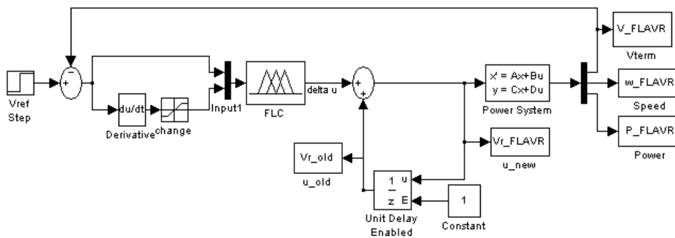
Fig. 5 SIMULINK diagram of the system with FLAVR
