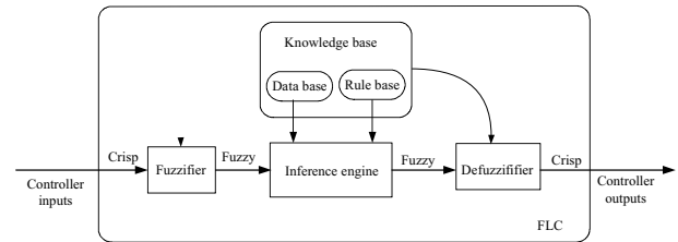
Fig. 1 Schematic diagram of the FLC building blocks
