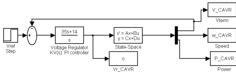
Fig. 3 SIMULINK diagram the system with CAVR
