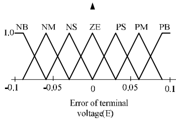
Fig. 6 Membership functions of terminal voltage error
