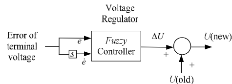
Fig. 4 Structure of the fuzzy logic based AVR
