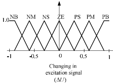
Fig. 8 Membership functions of excitation signal
