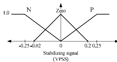
Fig. 14 Membership functions of stabilizing signal (VPSS)
