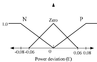
Fig. 12 Membership functions of power deviation (E)
