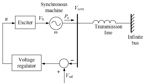
Fig. 2 Single-machine infinite-bus system
