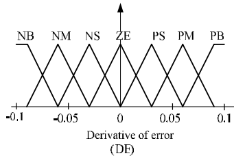
Fig. 7 Membership functions of terminal voltage error derivative
