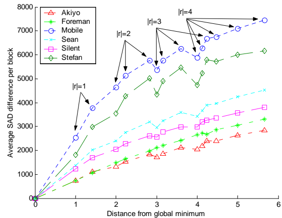
Fig. 2 Analysis of the relation between block SAD and distance
