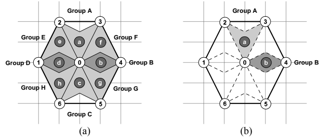
Fig. 5 (a) The new grouping for the hexagonal search pattern based on minimizing mean internal distance (MID). The eight inner points are separated into 2 sets by the MID value – Set-1: {a, c, e, f, g, h} and Set-2: {b, d}. (b) Point 'a' and 'b' are searched finally, because group A and group B have the smallest normalized group distortion in the corresponding set
