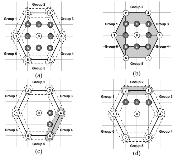
Fig. 1 Configurations and examples of the 6-side-based inner search; (a) groups of evaluated points; (b) defining shaded region for each group; (c) group 4 wins and checks point 'b' and 'g'; (d) group 2 wins and checks point 'a', 'e' and 'f'
