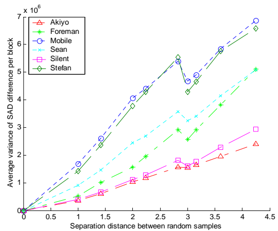
Fig. 3 Variance of block SAD difference for the random sample pairs taken from the 4 \times 4 region around the global minimum
