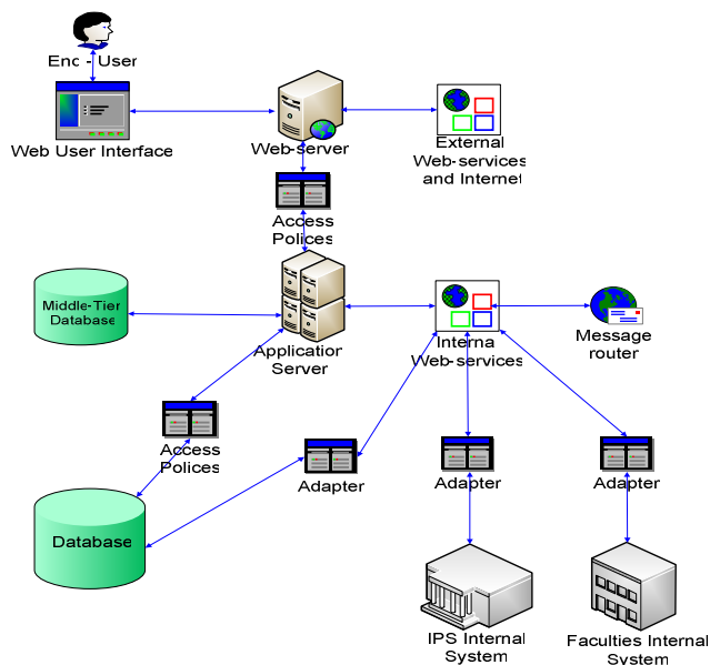
Fig. 1 Adopting development framework of Web-Services based on SOA
