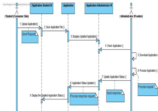
Fig. 2 MEPs sequence diagram for check application status services
