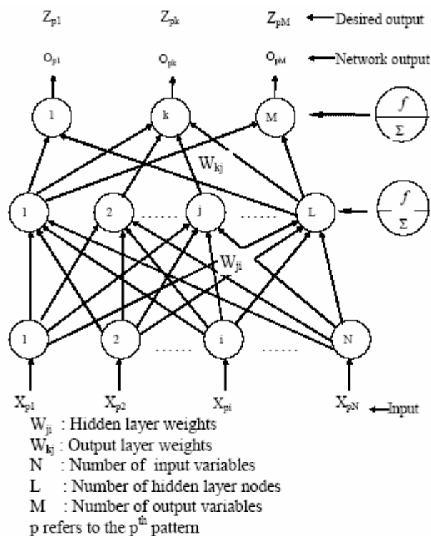
Fig. 1 Generic representation of the ANN of MLP
