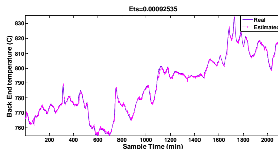
Fig. 5 Normal model with 5 min prediction horizon
