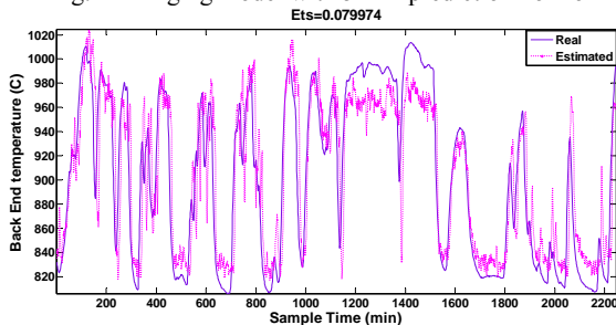
Fig. 13 Ringing model with 7 min prediction horizon
