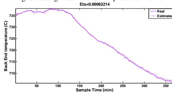
Fig. 9 Coating model with 5 min prediction horizon
