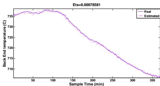
Fig. 10 Coating model with 7 min prediction horizon
