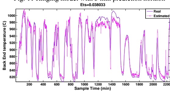
Fig. 12 Ringing model with 5 min prediction horizon
