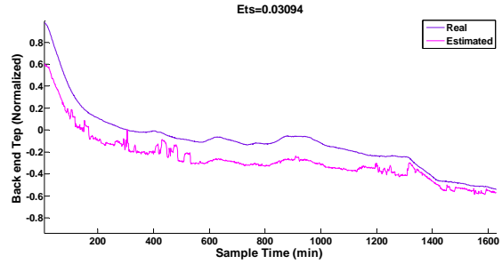
Fig. 20 Test of the normal model with the coating validity data
