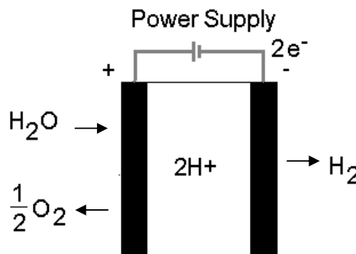
Fig. 3. Electrolyzer Component
