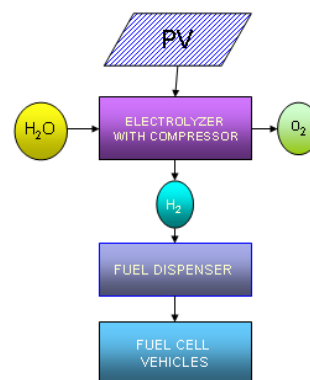
Fig. 1. PV-Electrolyzer System
