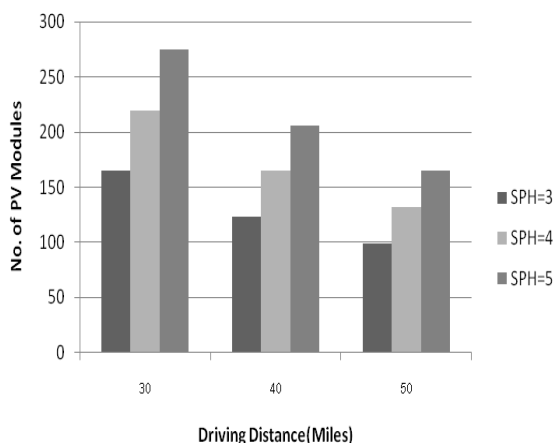
Fig. 5. Number of PV modules
