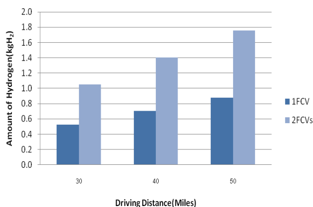
Fig. 4. Amount of Hydrogen for FCVs
