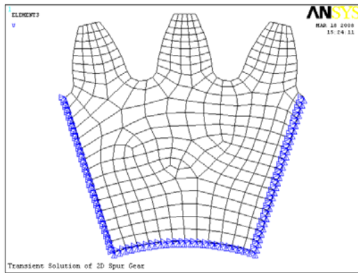
Fig. 2 Finite element mesh
