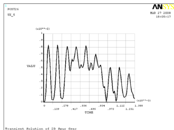
Fig. 7 Displacement of the model in X-Direction
