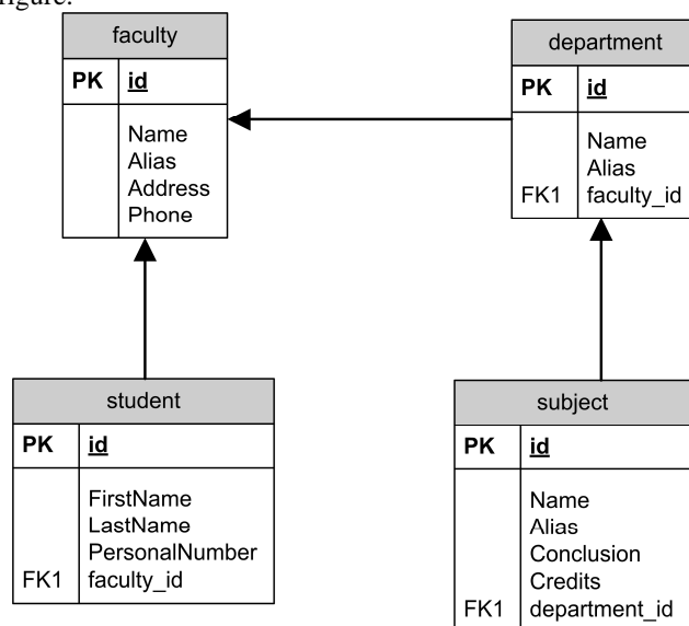
Fig. 4 Selected database logical structure
