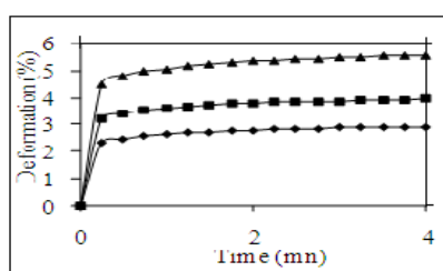
Fig. 5 Short-time creep curves for a foam middle
