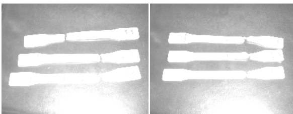
Fig. 1 Photos of tested LDPE specimens
