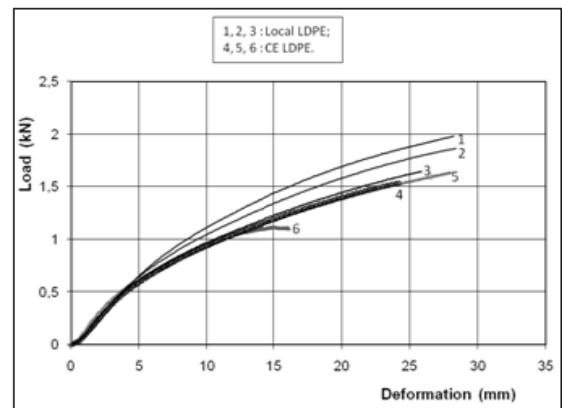
Fig. 3 Initial characterization of materials
