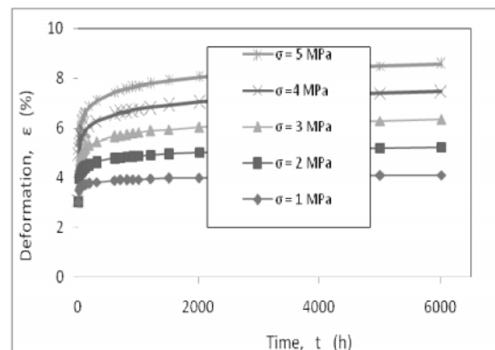
Fig. 9 Middle-time creep simulation for various values of axial stress "σ". (All mediums)
