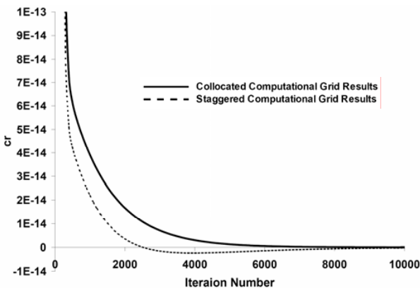
Fig. 2 cr (eq. 4) as a function of iteration number. In computational algorithm the program stops when cr extends to e .
