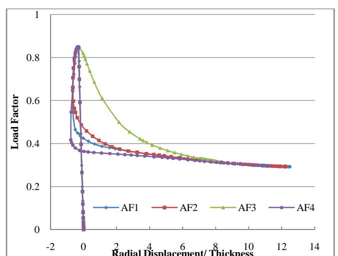
Fig. 9b Load factor versus radial displacement normalized with shell wall thickness for AMT 'AF'
