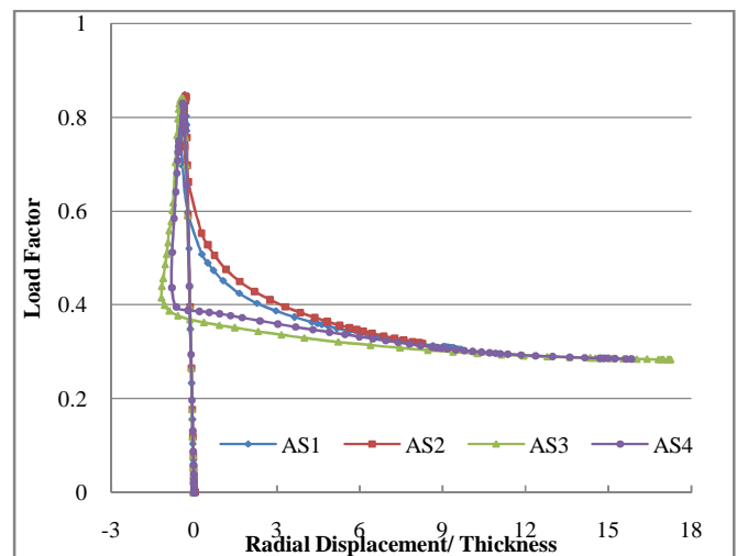
Fig. 10b Load factor versus radial displacement normalized with shell wall thickness for AMT 'AS'
