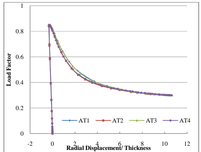
Fig. 8b Load factor versus radial displacement normalized with shell wall thickness for AMT 'AT'
