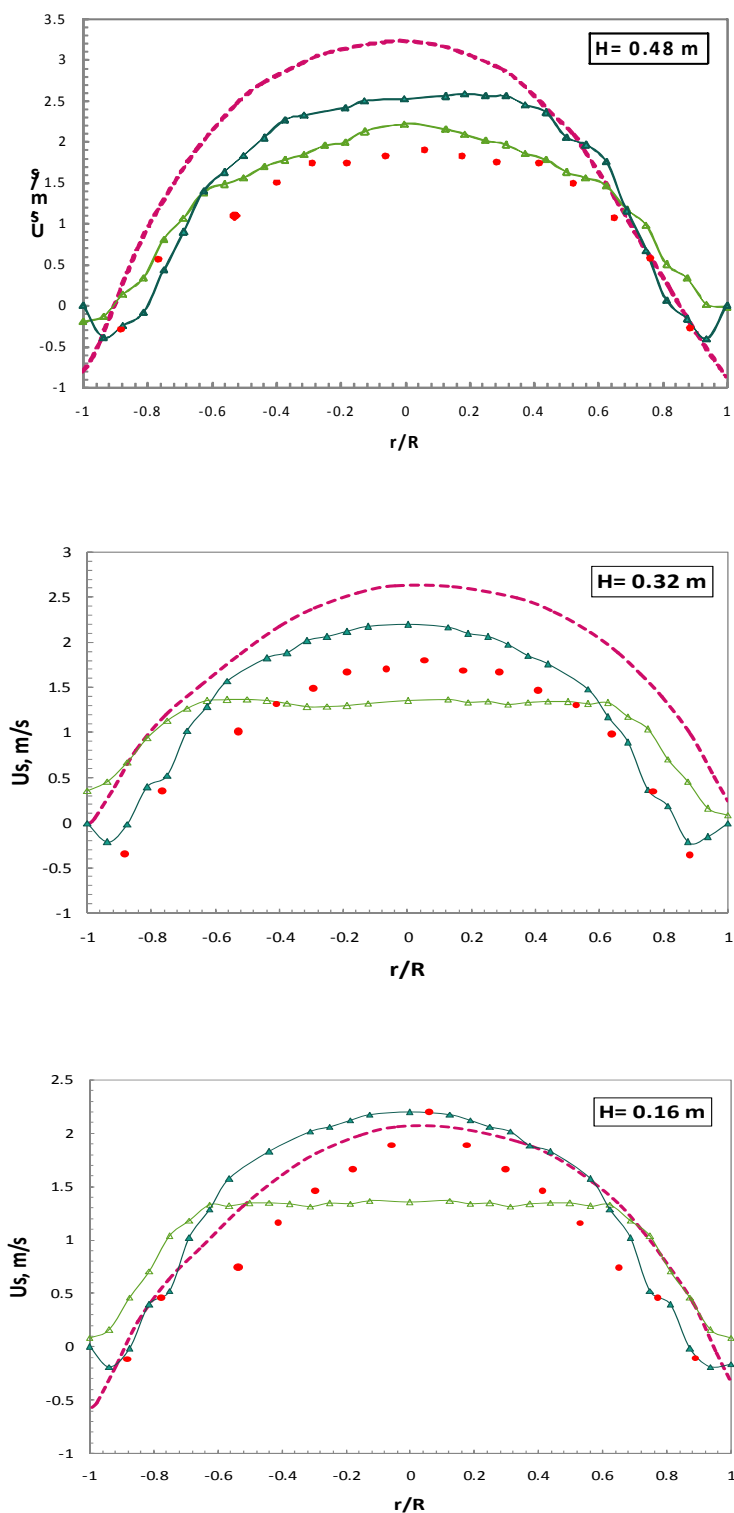
Fig. 2 Radial profiles of particle velocity along the riser different operating conditions, U_g=1.42 m/s. ● Experimental; --- [28]; -▲- No Slip; - \Delta - Free slip
