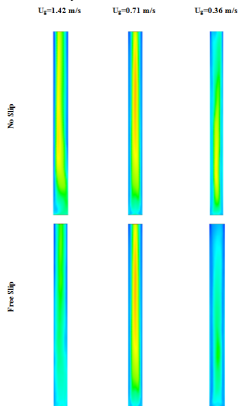
Fig 1 Average Courant Number at the center of the riser (XY plane): Free slip (top) and No-Slip (bottom).
