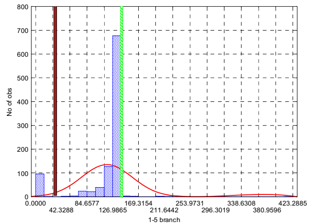
Fig. 3 Apparent power flow on branch 1-5
