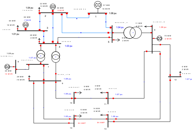
Fig. 2 IEEE 14 bus test power system configuration scheme
