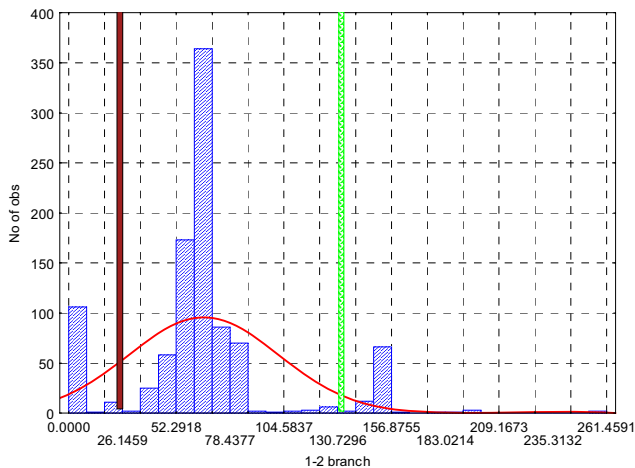
Fig. 4 Apparent power flow on branch 1-2
