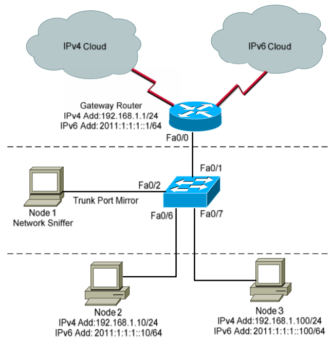
Fig. 3 Testbed network layout
