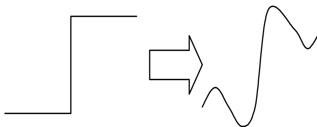
FIGURE IV. 1-D RINGING EFFECT CAUSED BY OVER-COMPRESSION
