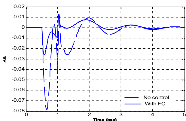
Fig. 14 DFIG slip variation following a three-phase 0.5s fault with and without proposed frequency controller
