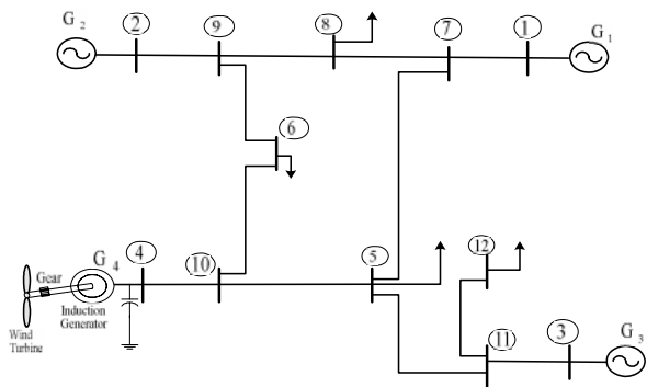
Fig. 6 Multimachine system configuration including asynchronous machine
